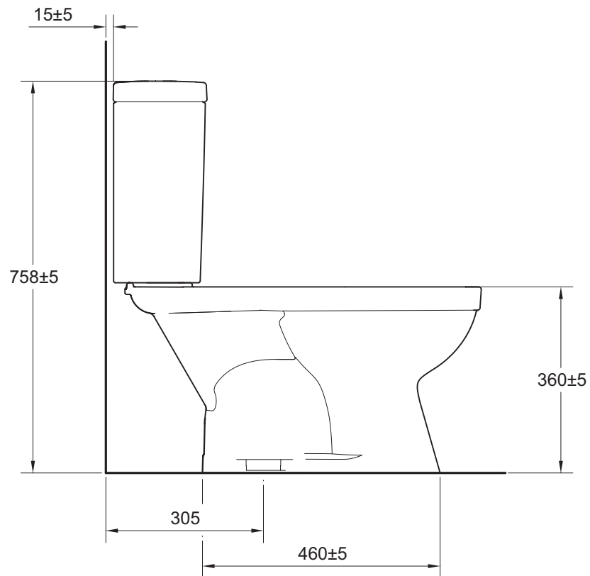
SIDE VIEW
